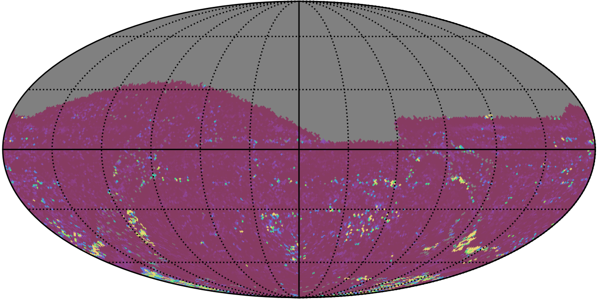
ddf_acor_sf10_lsf30_lsr50_v3.4_10yrs All sky g band: 75th Percentile Intranight Timespan
