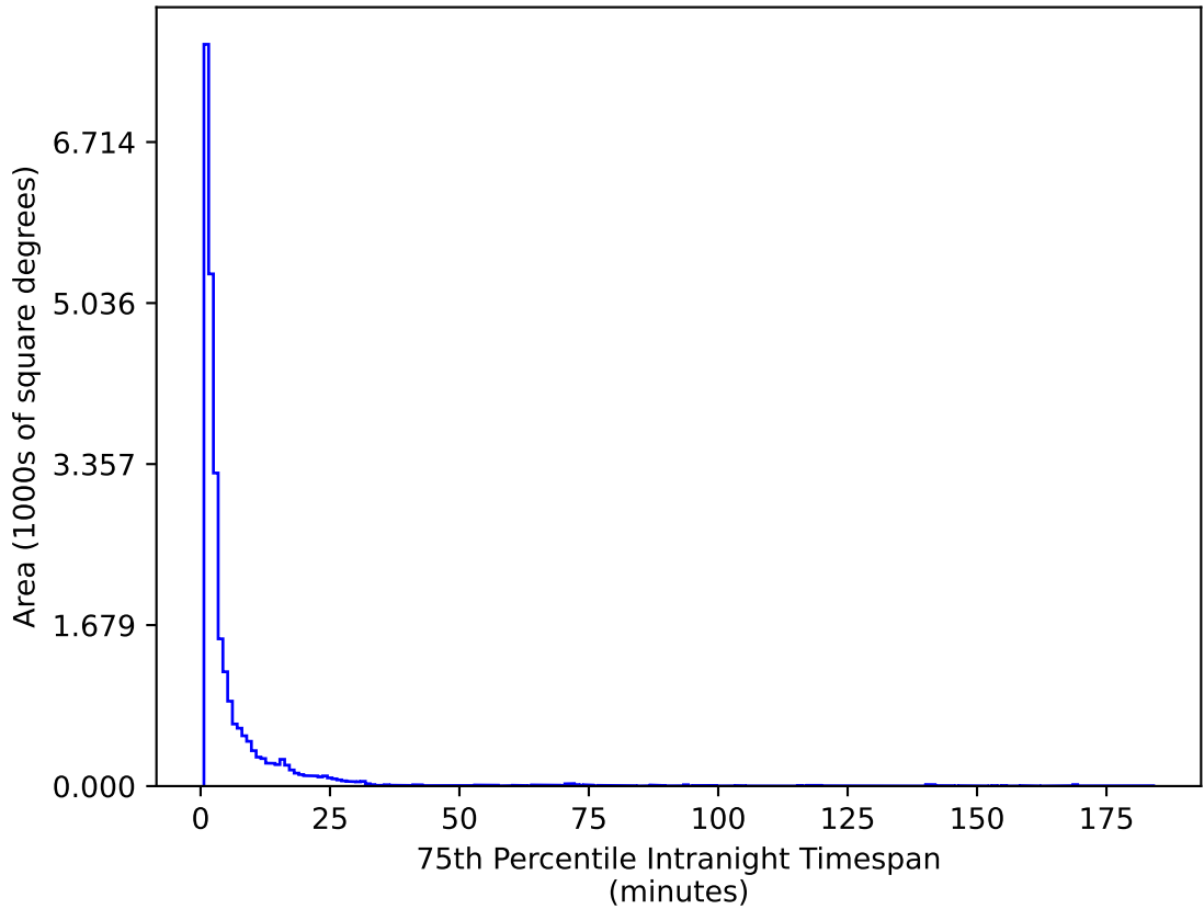
ddf_acor_sf10_lsf30_lsr50_v3.4_10yrs All sky g band: 75th Percentile Intranight Timespan
