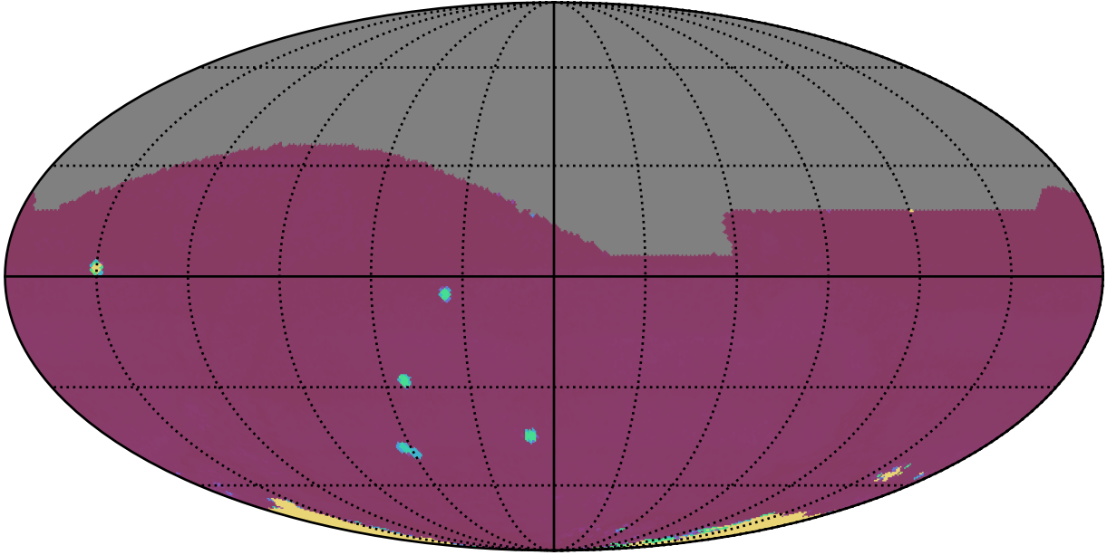
ddf_acor_sf10_lsf30_lsr50_v3.4_10yrs All sky all bands: 75th Percentile Intranight Timespan
