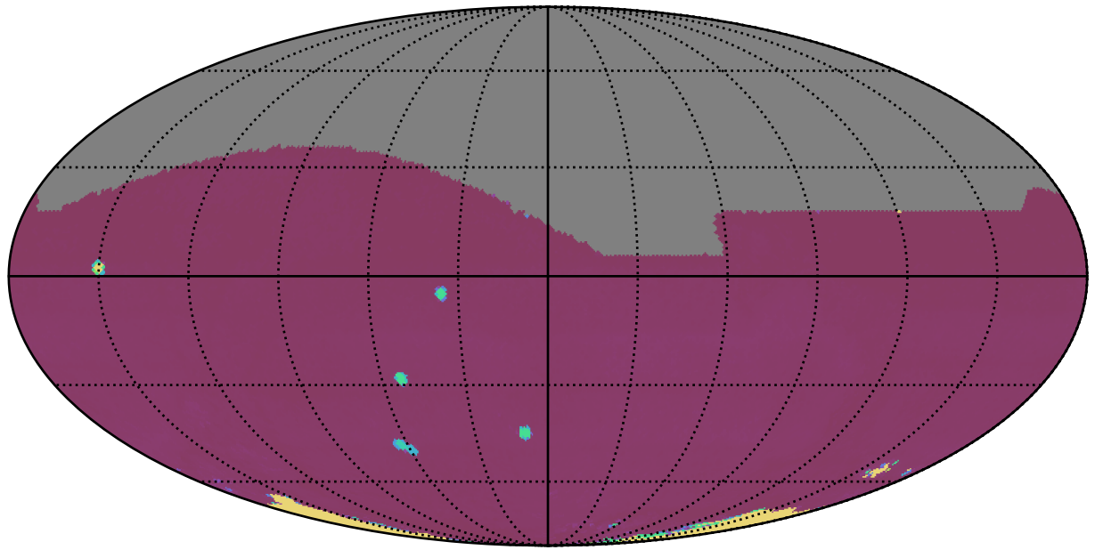
ddf_acor_sf10_lsf30_lsr50_v3.4_10yrs All sky: 75th Percentile Intranight Timespan
