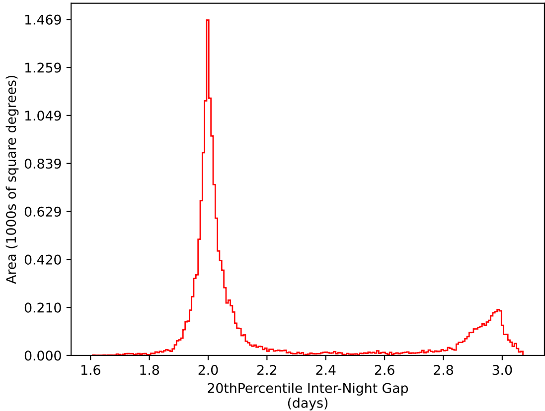
ddf_acor_sf10_lsf30_lsr50_v3.4_10yrs WFD i band: 20thPercentile Inter-Night Gap
