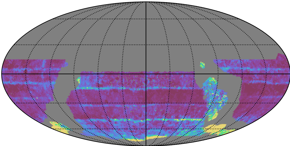
ddf_acor_sf10_lsf30_lsr50_v3.4_10yrs WFD all bands: 20thPercentile Inter-Night Gap
