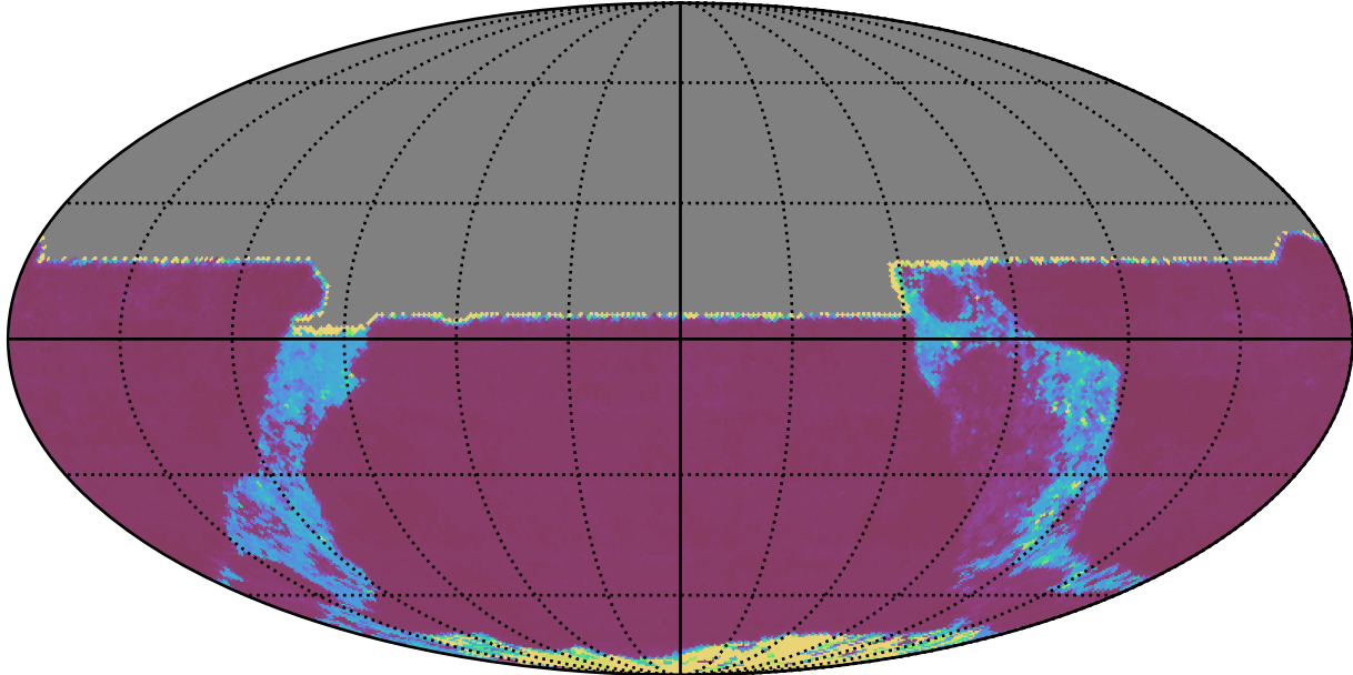
ddf_acor_sf10_lsf30_lsr50_v3.4_10yrs All sky y band: 20thPercentile Inter-Night Gap
