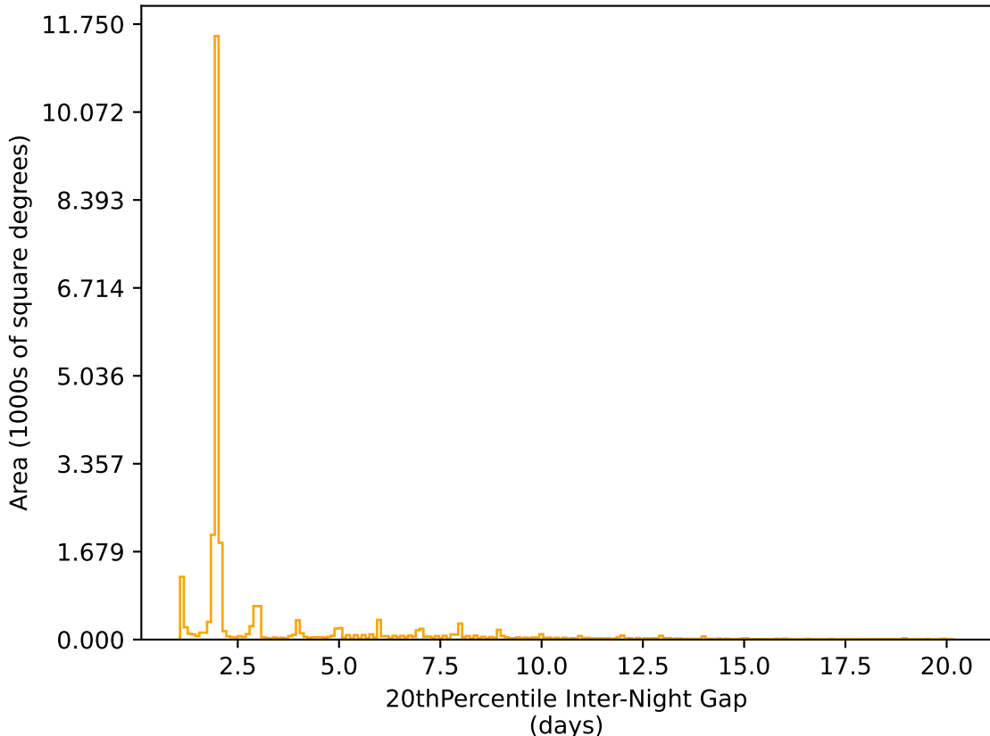
ddf_acor_sf10_ls30_lsr50_v3.4_10yrs All sky r band: 20thPercentile Inter-Night Gap
