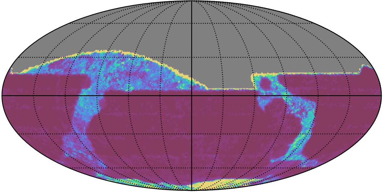
ddf_acor_sf10_lsf30_lsr50_v3.4_10yrs All sky i band: 20thPercentile Inter-Night Gap
