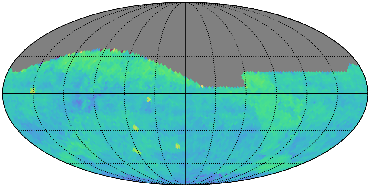
ddf_acor_sf10_lsf30_lsr50_v3.4_10yrs (g or r or i): PairFraction
