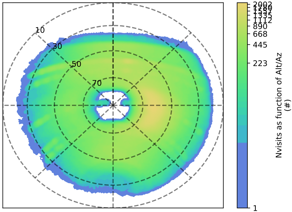
ddf_acor_sf10_lsf30_lsr50_v3.4_10yrs y: Nvisits as function of Alt/Az
