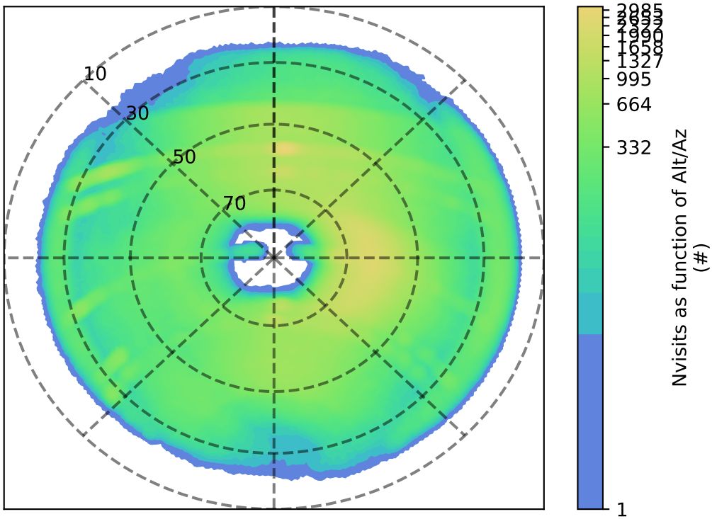
ddf_acor_sf10_ls30_lsr50_v3.4_10yrs i: Nvisits as function of Alt/Az
