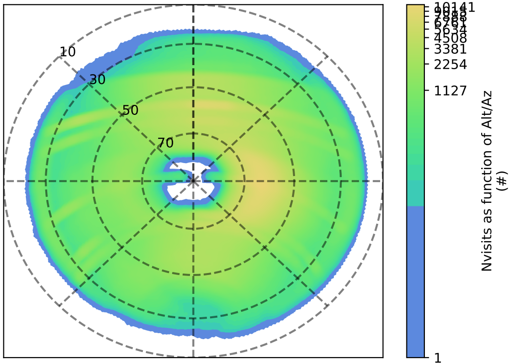
ddf_acor_sf10_lsf30_lsr50_v3.4_10yrs : Nvisits as function of Alt/Az
