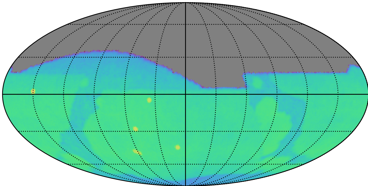
ddf_acor_sf10_lsf30_lsr50_v3.4_10yrs g: CoaddM5
