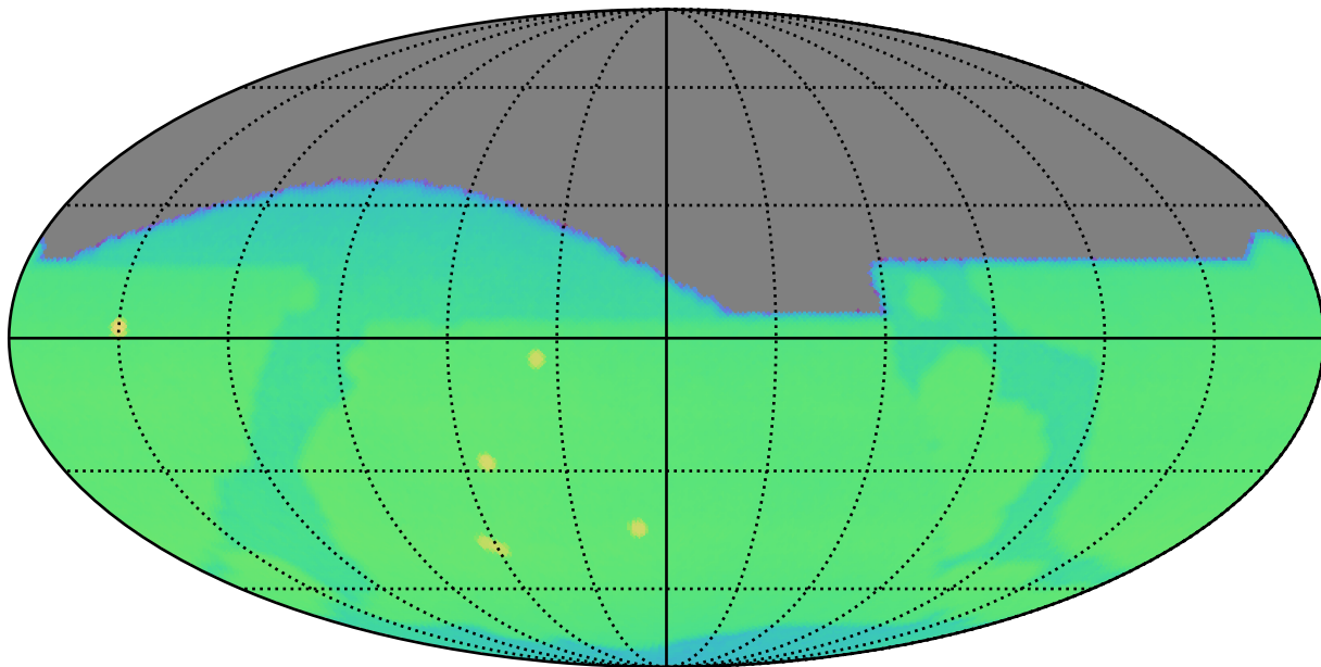
ddf_acor_sf10_lsf30_lsr50_v3.4_10yrs : CoaddM5
