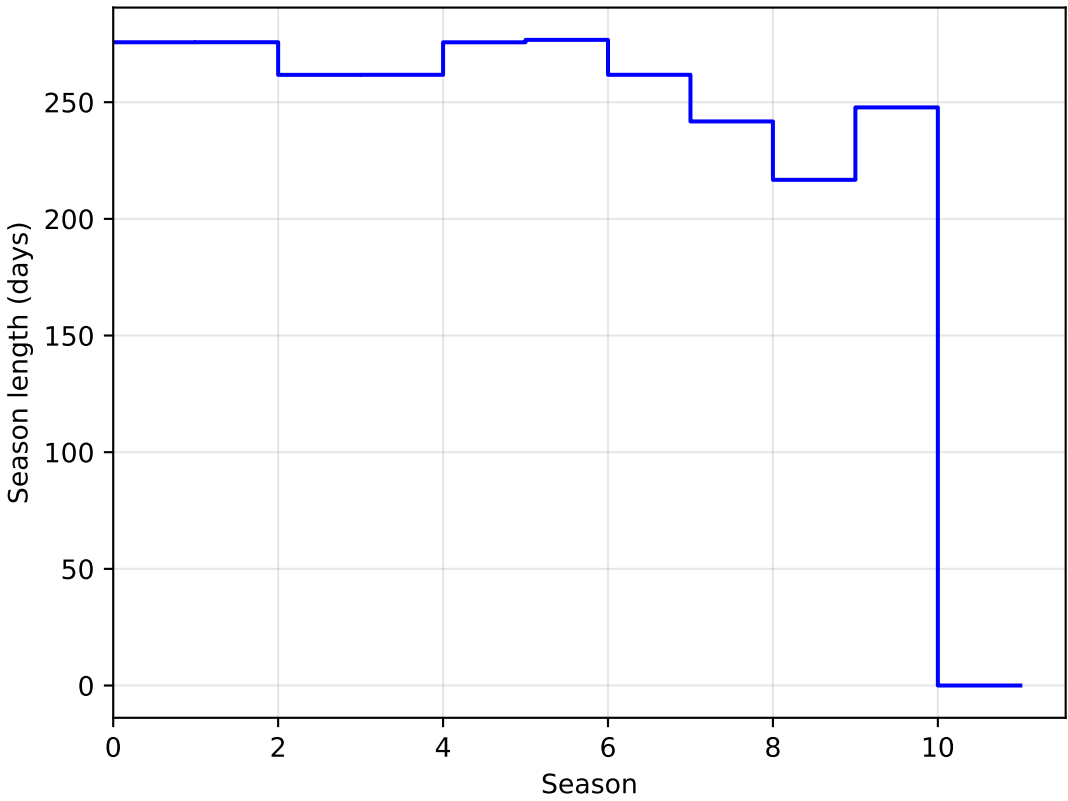
ddf_acor_sf10_lsf30_lsr50_v3.4_10yrs DD:EDFS all bands: SeasonLength
