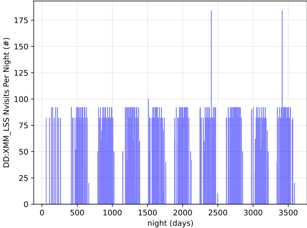
ddf_acor_sf10_lsf30_lsr50_v3.4_10yrs all bands: DD:XMM_LSS Nvisits Per Night
