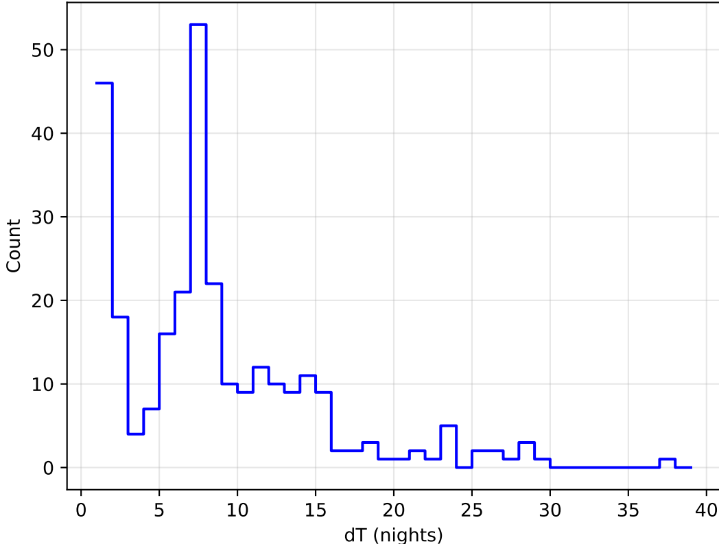
ddf_acor_sf10_lsf30_lsr50_v3.4_10yrs all bands: DD:XMM_LSS Delta Nights Histogram
