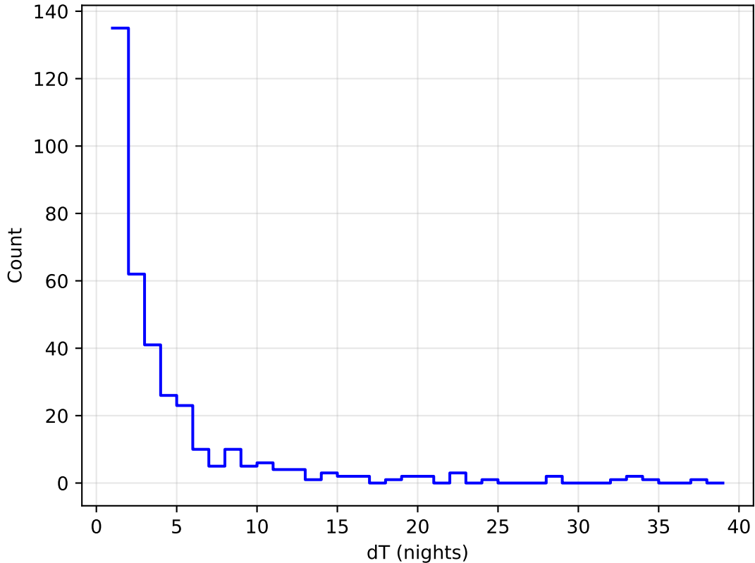
ddf_acor_sf10_lsf30_lsr50_v3.4_10yrs all bands: DD:WFD Delta Nights Histogram
