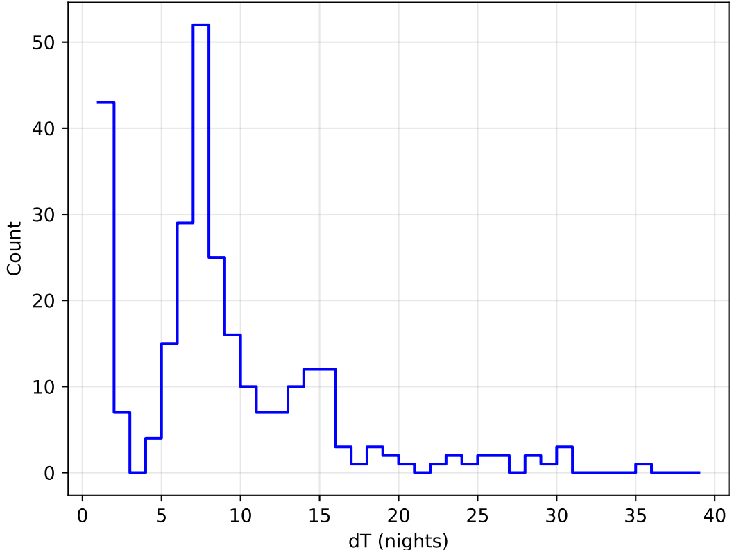
ddf_acor_sf10_lsf30_lsr50_v3.4_10yrs all bands: DD:ELAISS1 Delta Nights Histogram
