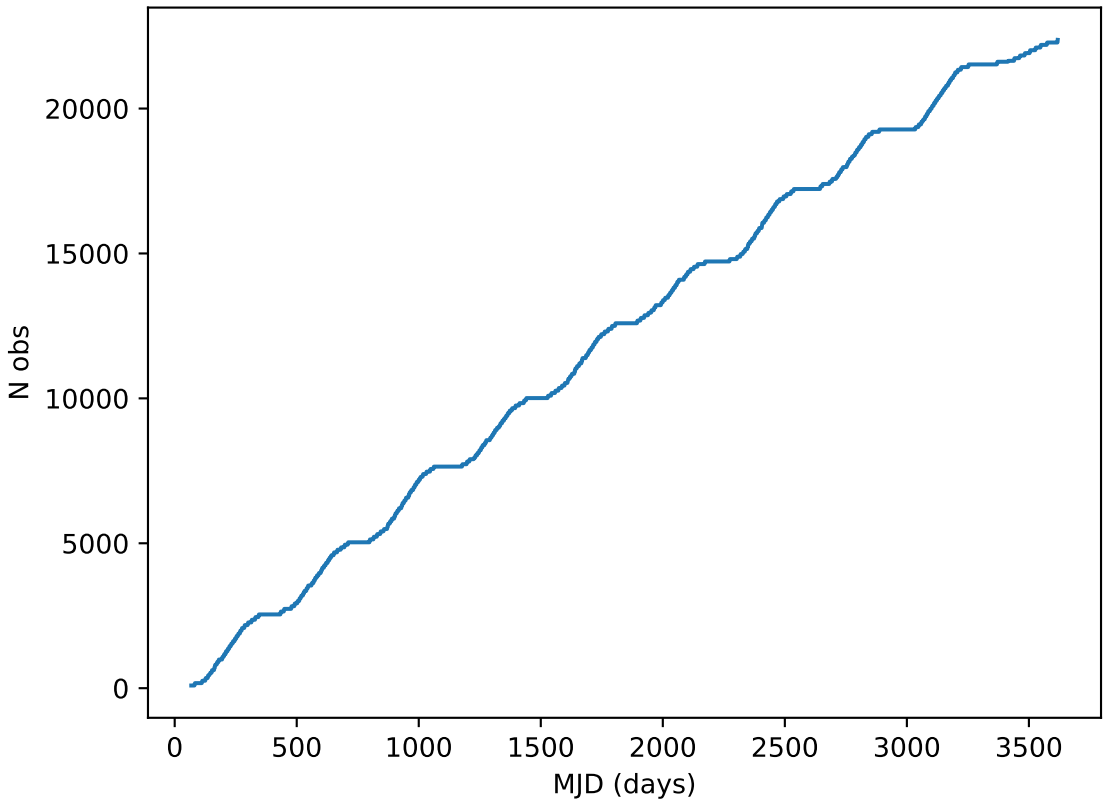
ddf_acor_sf10_lsf30_lsr50_v3.4_10yrs all bands: DD:EDFS Cumulative NVisits
