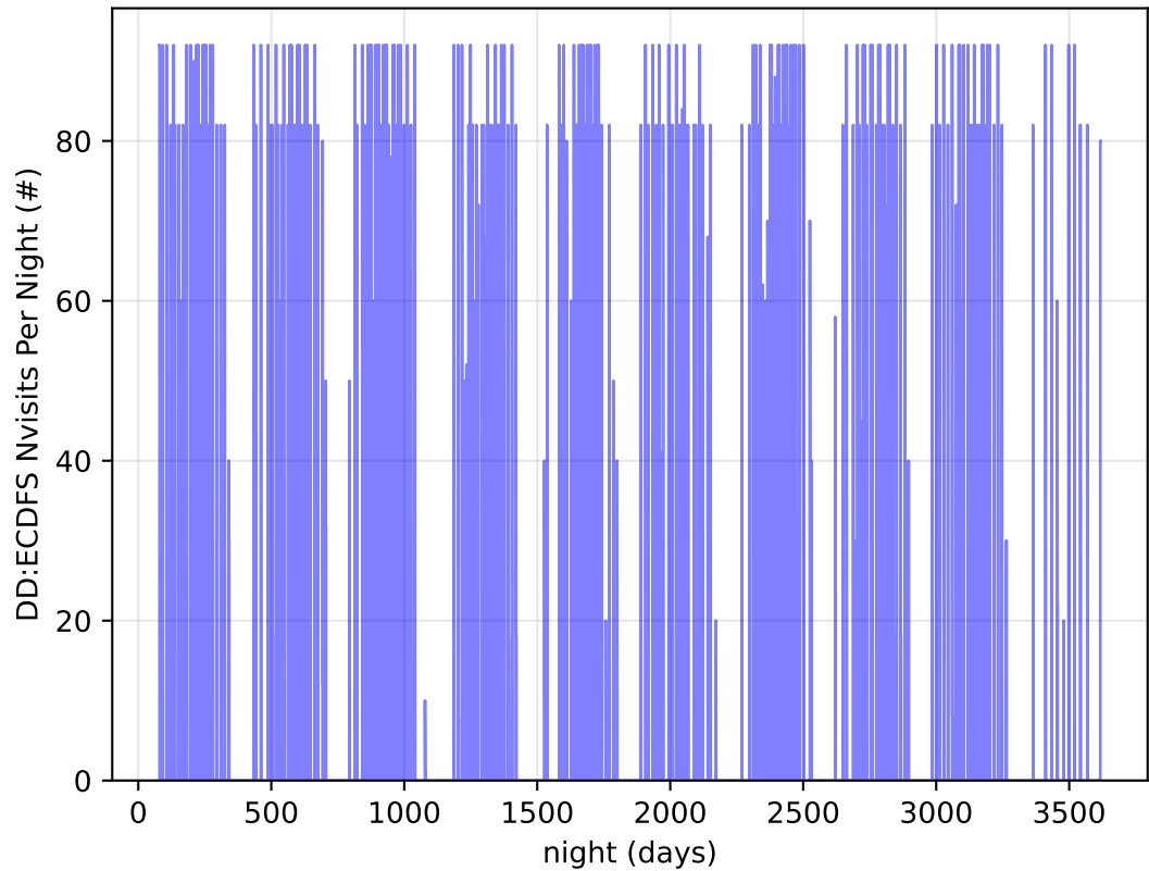
ddf_acor_sf10_lsf30_lsr50_v3.4_10yrs all bands: DD:ECDFS Nvisits Per Night
