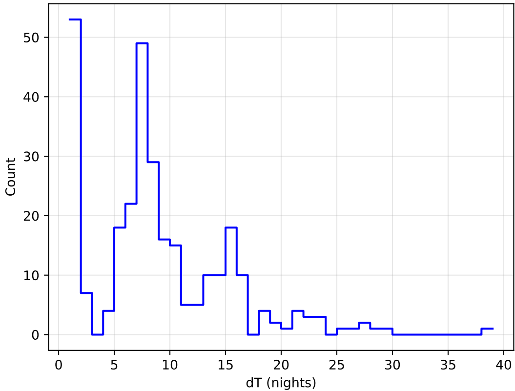
ddf_acor_sf10_lsf30_lsr50_v3.4_10yrs all bands: DD:ECDFS Delta Nights Histogram
