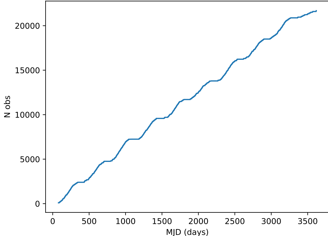
ddf_acor_sf10_lsf30_lsr50_v3.4_10yrs all bands: DD:ECDFS Cumulative NVisits
