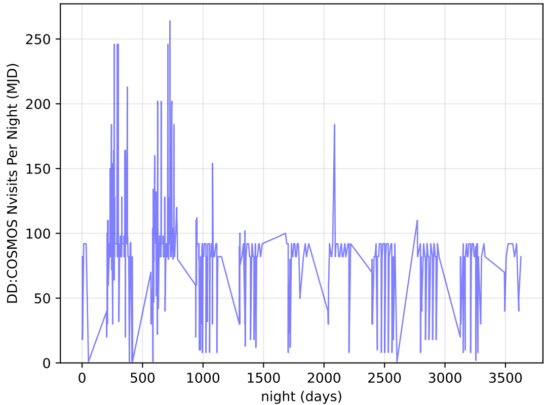
ddf_acor_sf10_lsf30_lsr50_v3.4_10yrs all bands: DD: COSMOS Nvisits Per Night
