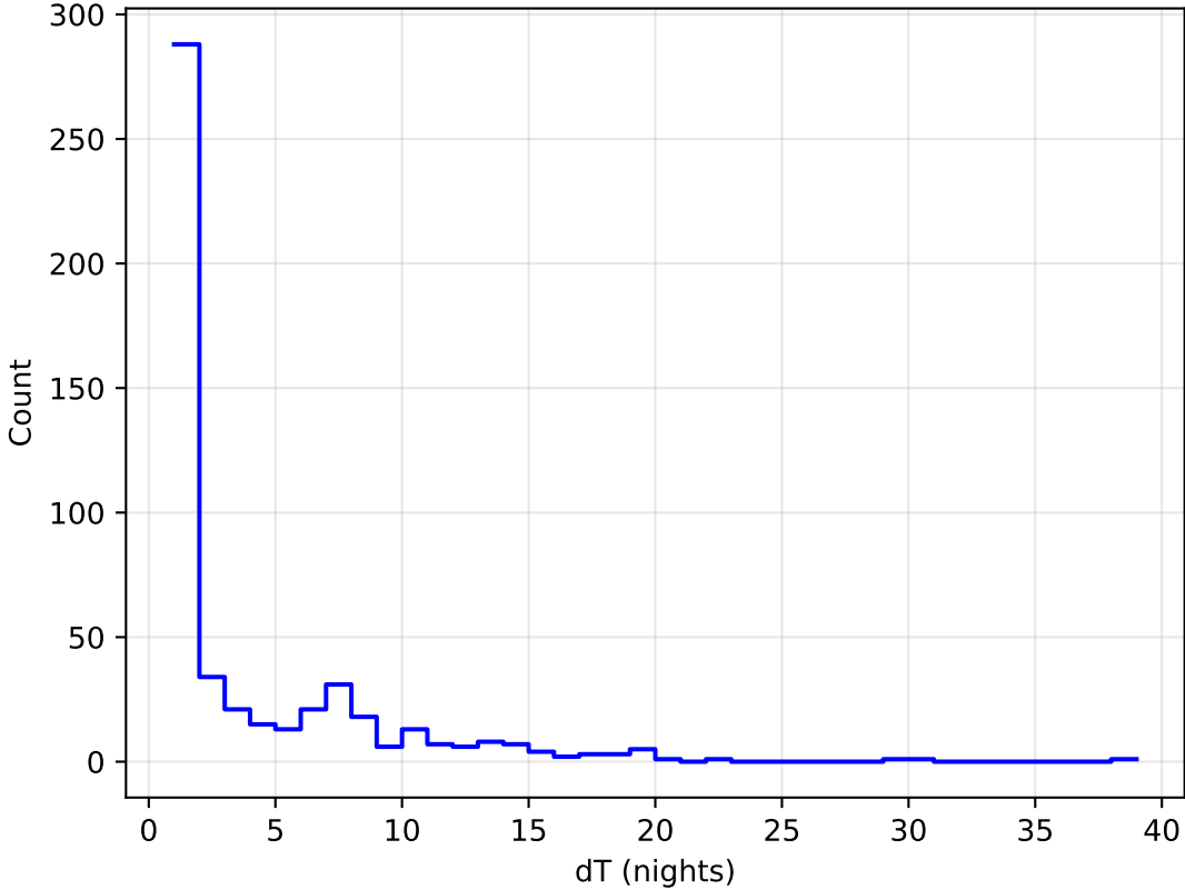
ddf_acor_sf10_Isf30_Isr50_v3.4_10yrs all bands: DD:COSMOS Delta Nights Histogram
