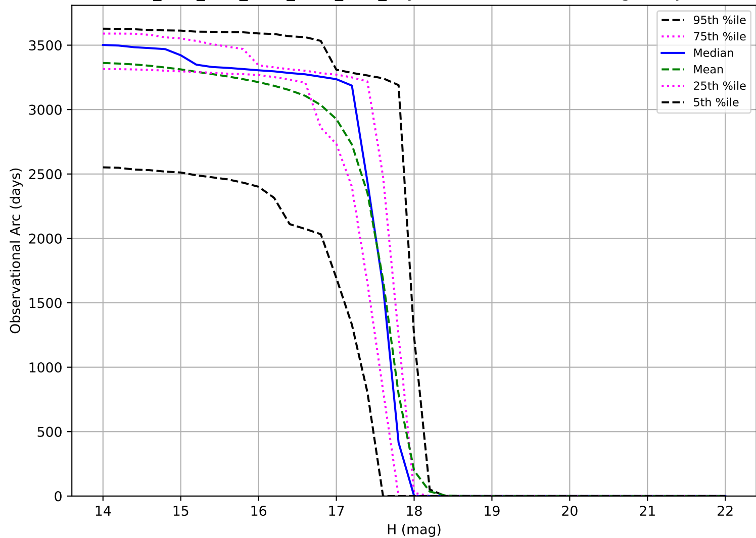
ddf_acor_sf10_lsf30_lsr20_v3.4_10yrs: Observational Arc Length Trojan
