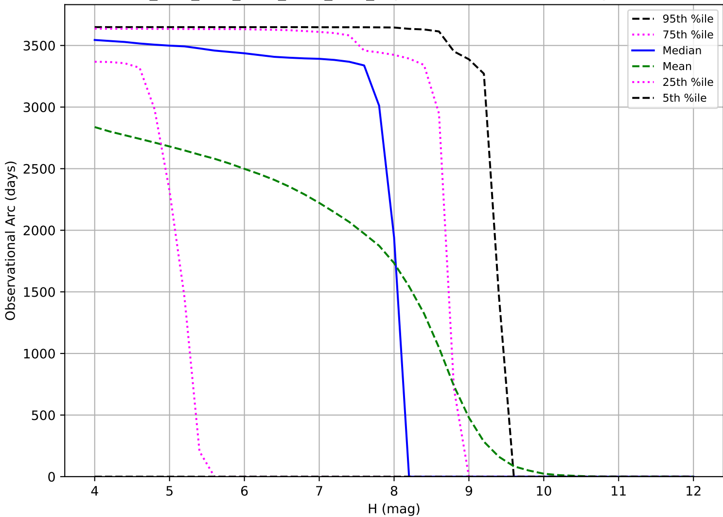
ddf_acor_sf10_Isf30_Isr20_v3.4_10yrs: Observational Arc Length TNO
