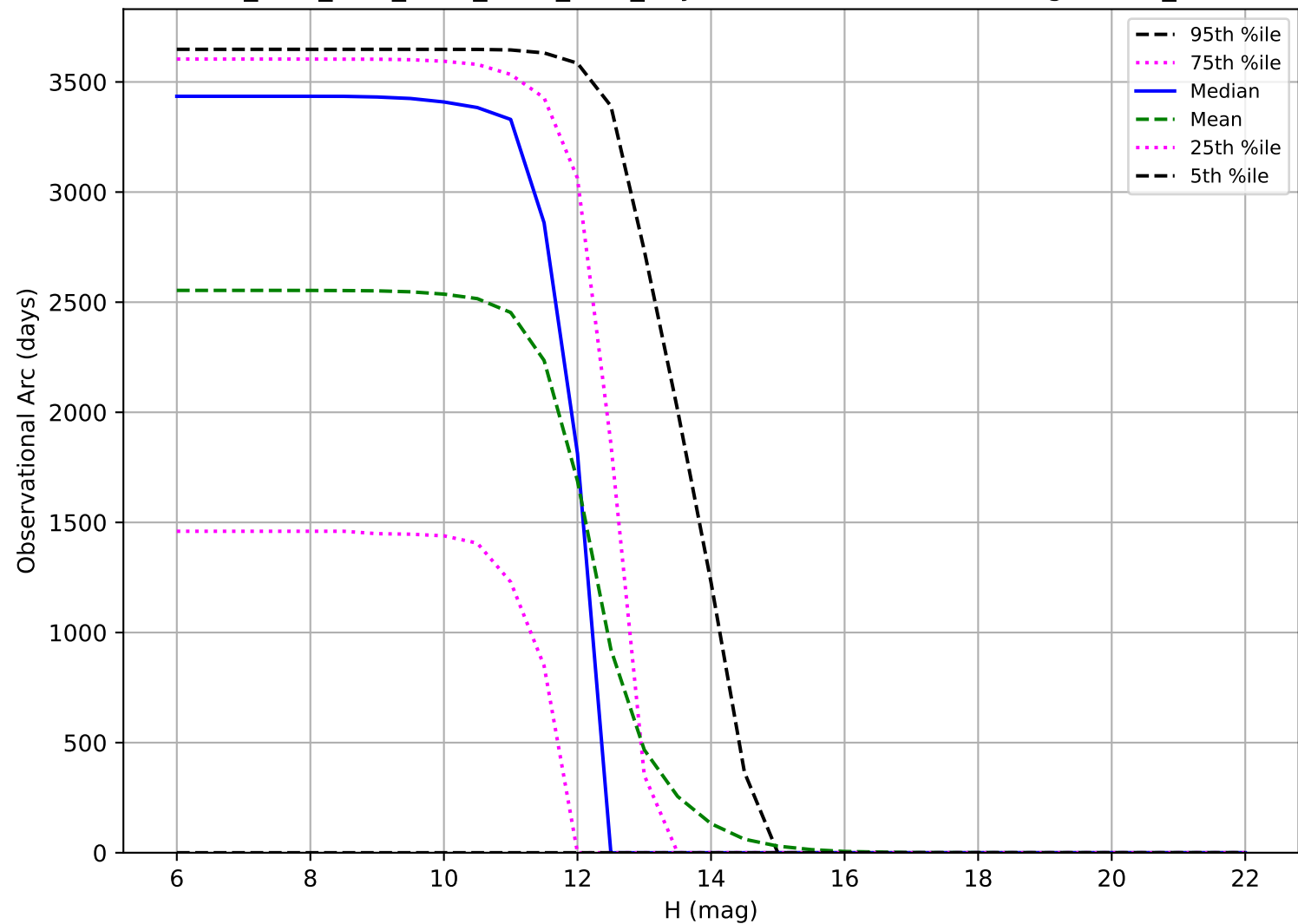
ddf_acor_sf10_lsf30_lsr20_v3.4_10yrs: Observational Arc Length OCC_r20
