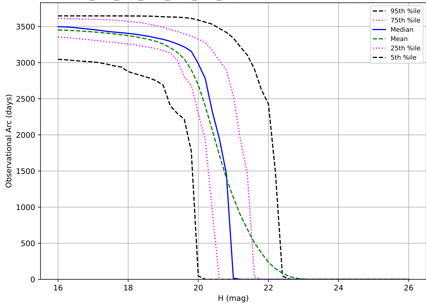
ddf_acor_sf10_lsf30_lsr20_v3.4_10yrs: Observational Arc Length MBA
