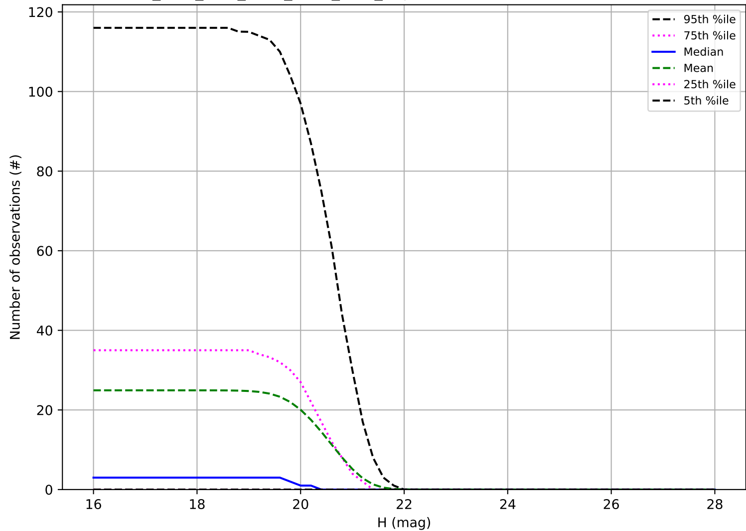
ddf_acor_sf10_lsf30_lsr20_v3.4_10yrs: Number of observations Vatira
