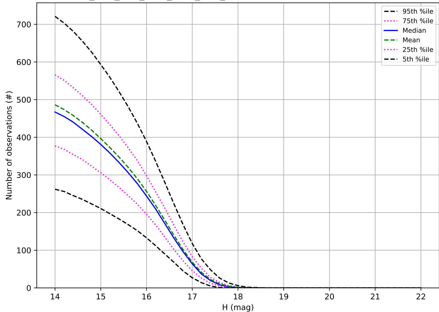
ddf_acor_sf10_lsf30_lsr20_v3.4_10yrs: Number of observations Trojan
