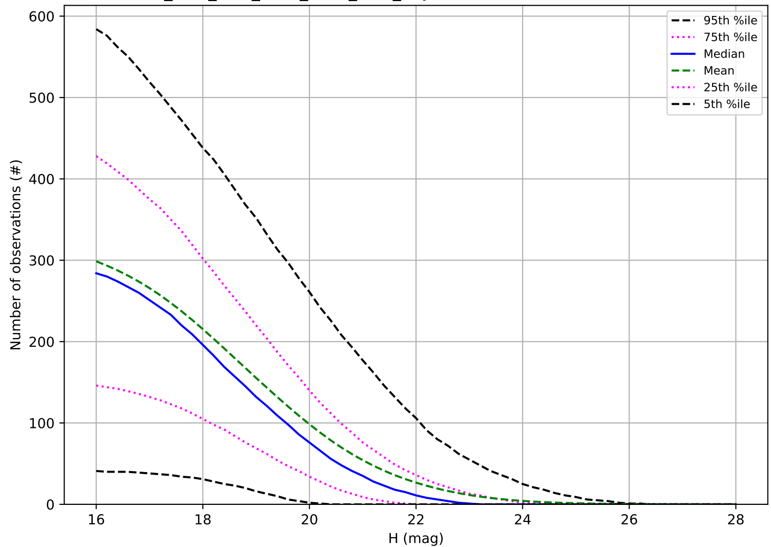
ddf_acor_sf10_lsf30_lsr20_v3.4_10yrs: Number of observations PHA
