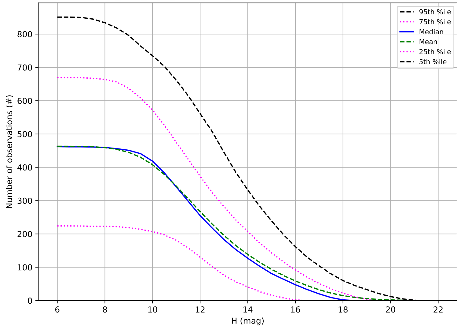
ddf_acor_sf10_lsf30_lsr20_v3.4_10yrs: Number of observations OCC_r5
