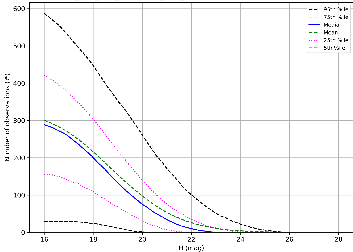
ddf_acor_sf10_lsf30_lsr20_v3.4_10yrs: Number of observations NEO
