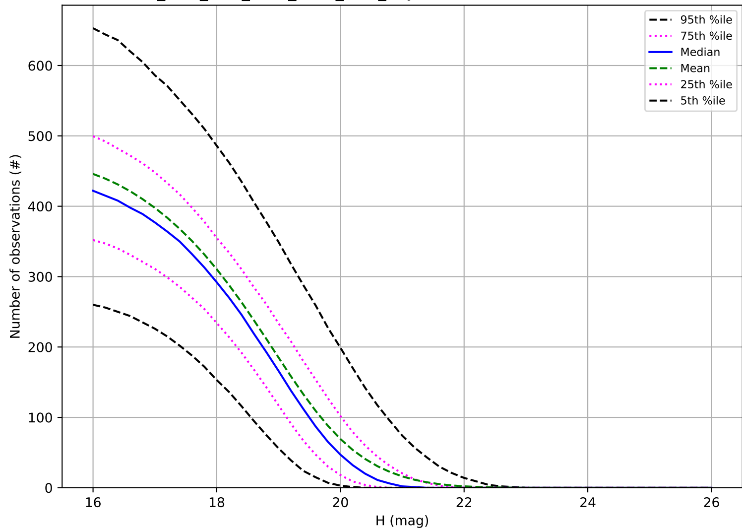
ddf_acor_sf10_lsf30_lsr20_v3.4_10yrs: Number of observations MBA
