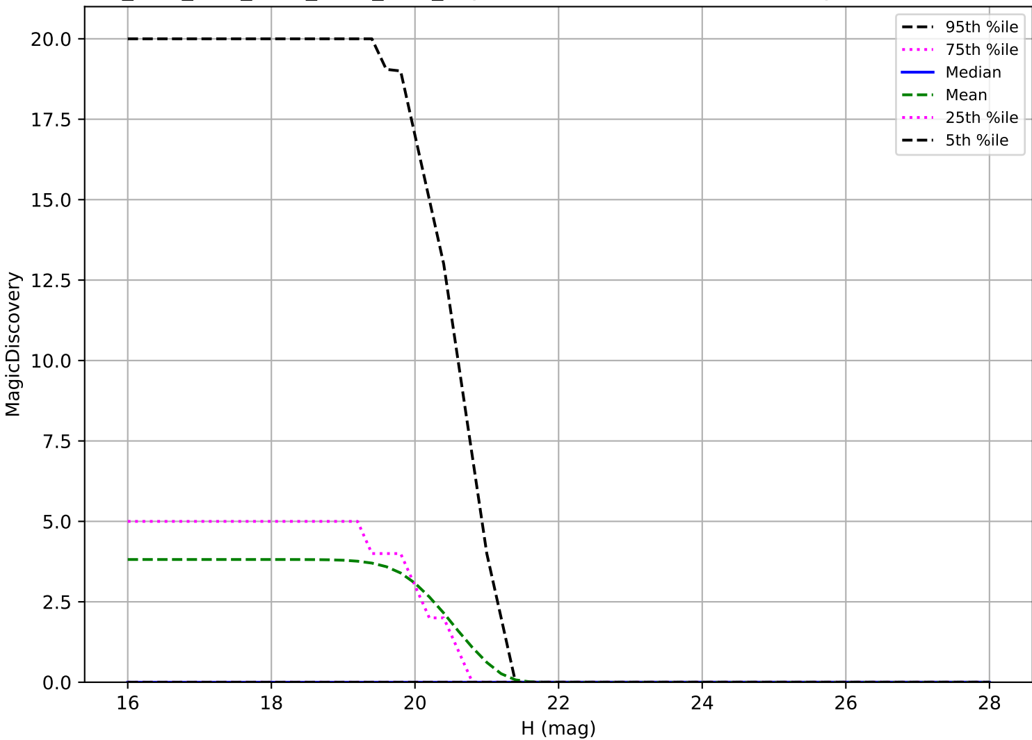
ddf_acor_sf10_lsf30_lsr20_v3.4_10yrs: Vatira 6 detections in 60 nights detection loss
