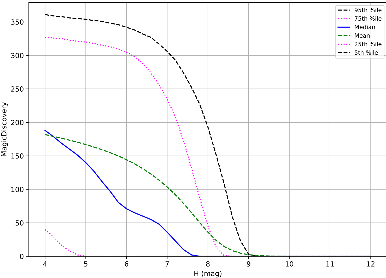
ddf_acor_sf10_lsf30_lsr20_v3.4_10yrs: TNO 6 detections in 60 nights detection loss
