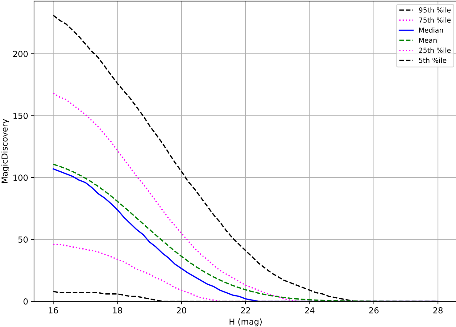
ddf_acor_sf10_lsf30_lsr20_v3.4_10yrs: PHA 6 detections in 60 nights detection loss
