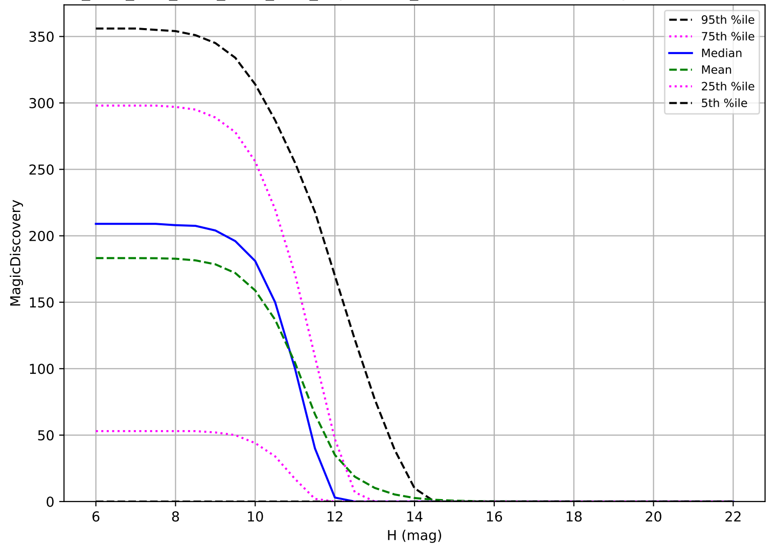
ddf_acor_sf10_lsf30_lsr20_v3.4_10yrs: OCC_r20 6 detections in 60 nights detection loss
