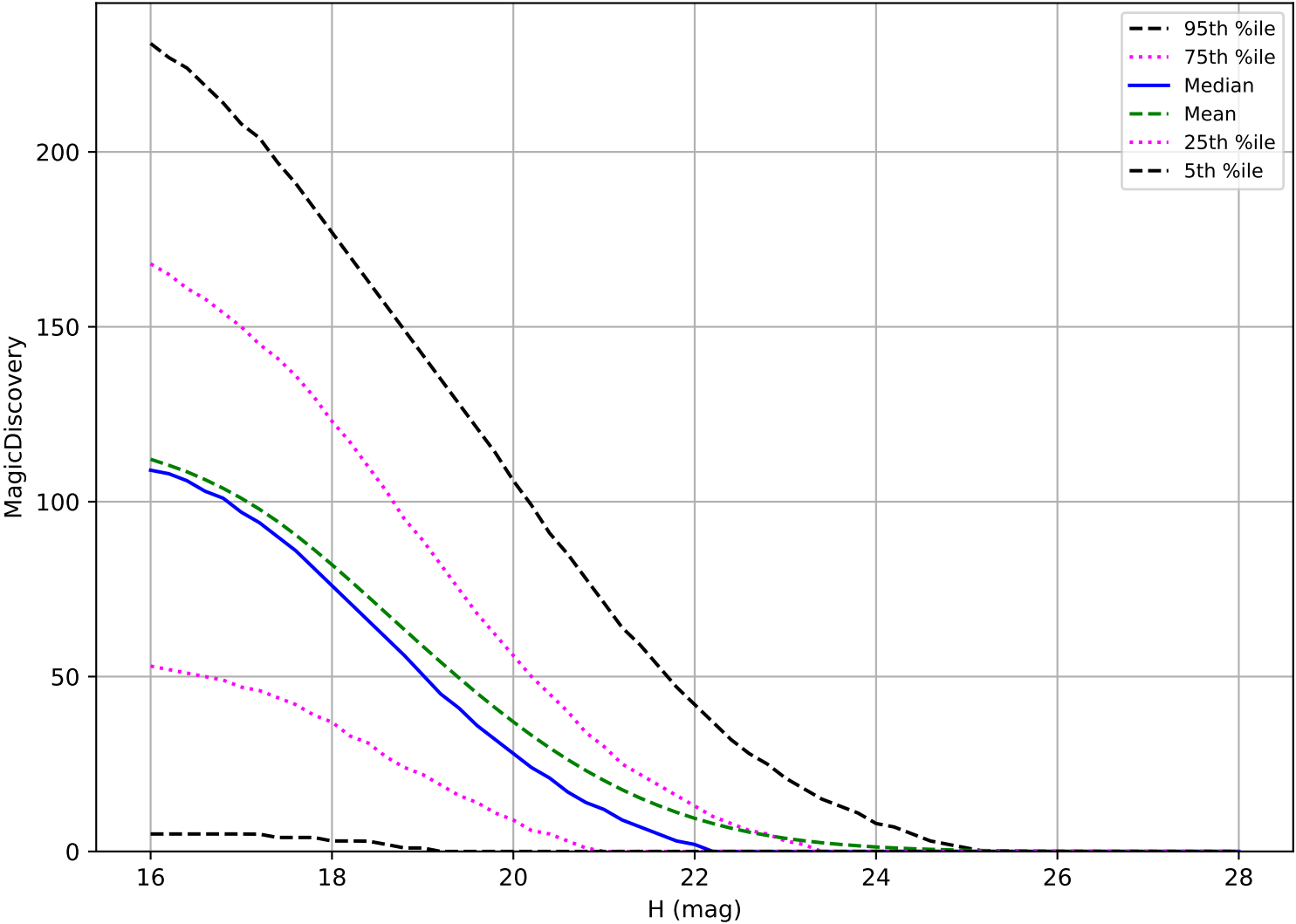
ddf_acor_sf10_lsf30_lsr20_v3.4_10yrs: NEO 6 detections in 60 nights detection loss
