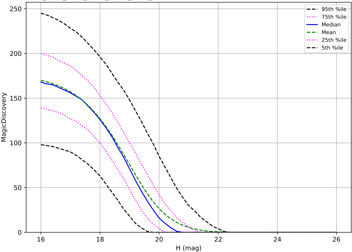
ddf_acor_sf10_lsf30_lsr20_v3.4_10yrs: MBA 6 detections in 60 nights detection loss
