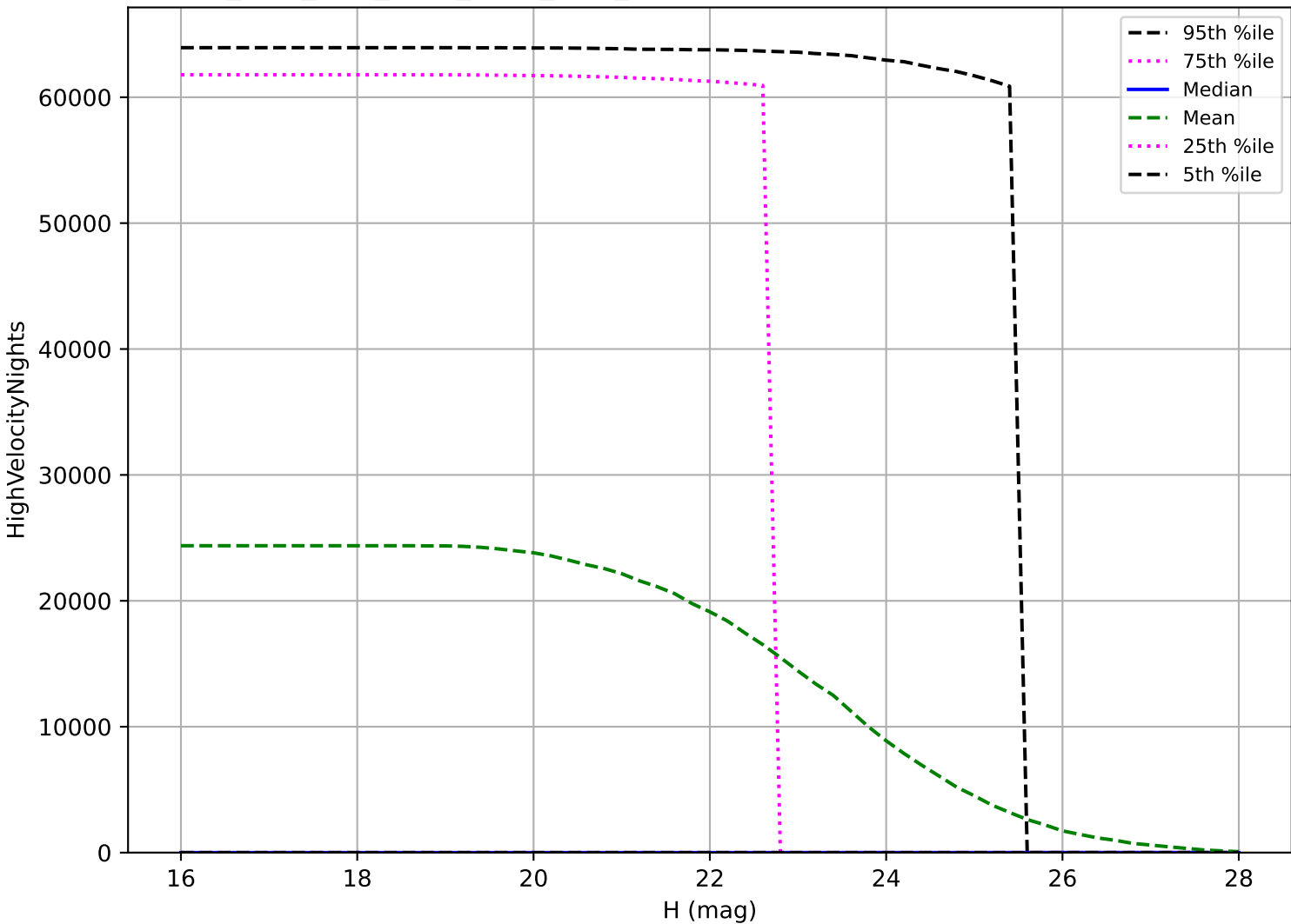
ddf_acor_sf10_lsf30_lsr20_v3.4_10yrs: PHA High velocity pair detection loss
