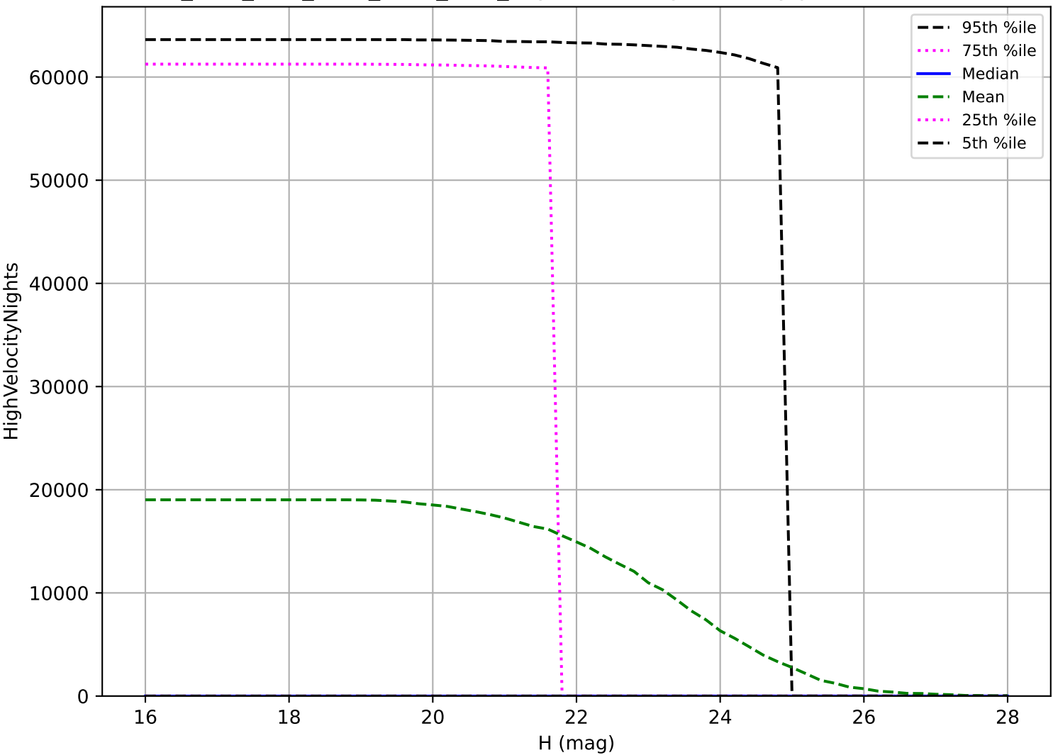
ddf_acor_sf10_lsf30_lsr20_v3.4_10yrs: NEO High velocity pair detection loss
