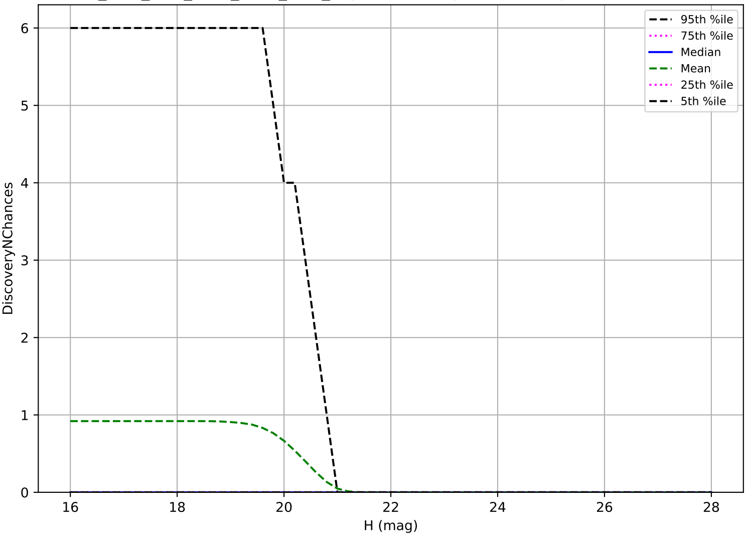
ddf_acor_sf10_lsf30_lsr20_v3.4_10yrs: Vatira 3 pairs in 15 nights detection loss
