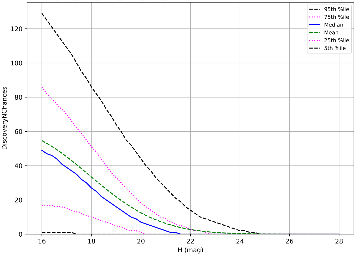
ddf_acor_sf10_lsf30_lsr20_v3.4_10yrs: PHA 3 pairs in 15 nights detection loss
