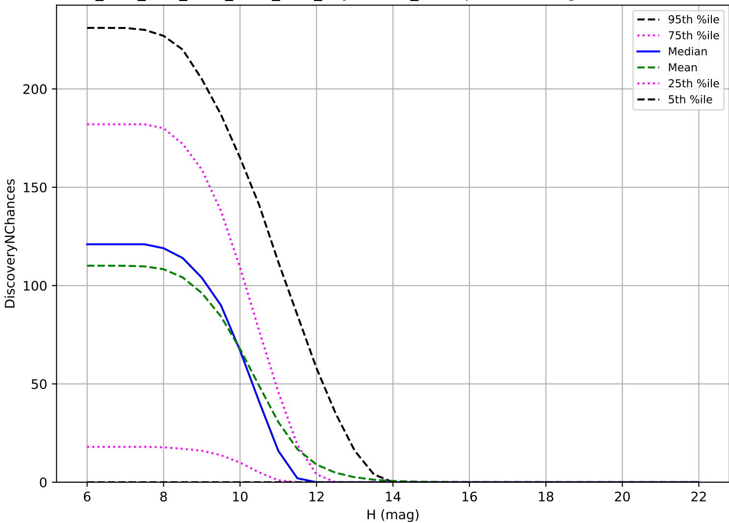
ddf_acor_sf10_lsf30_lsr20_v3.4_10yrs: OCC_r20 3 pairs in 15 nights detection loss
