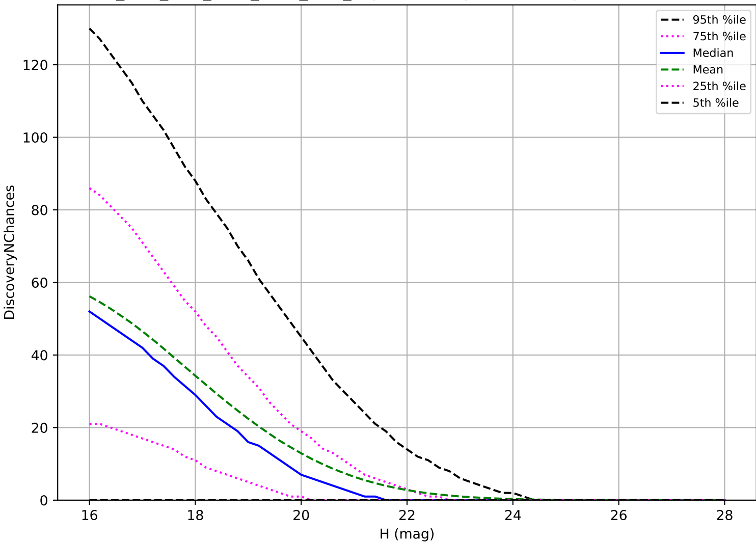
ddf_acor_sf10_lsf30_lsr20_v3.4_10yrs: NEO 3 pairs in 15 nights detection loss
