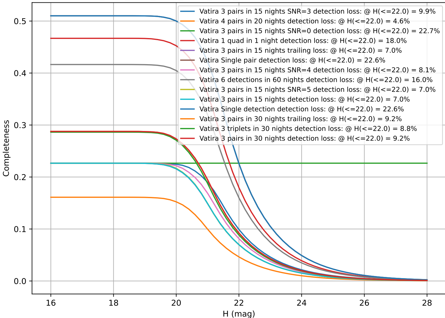
ddf_acor_sf10_lsf30_lsr20_v3.4_10yrs: CumulativeCompleteness
