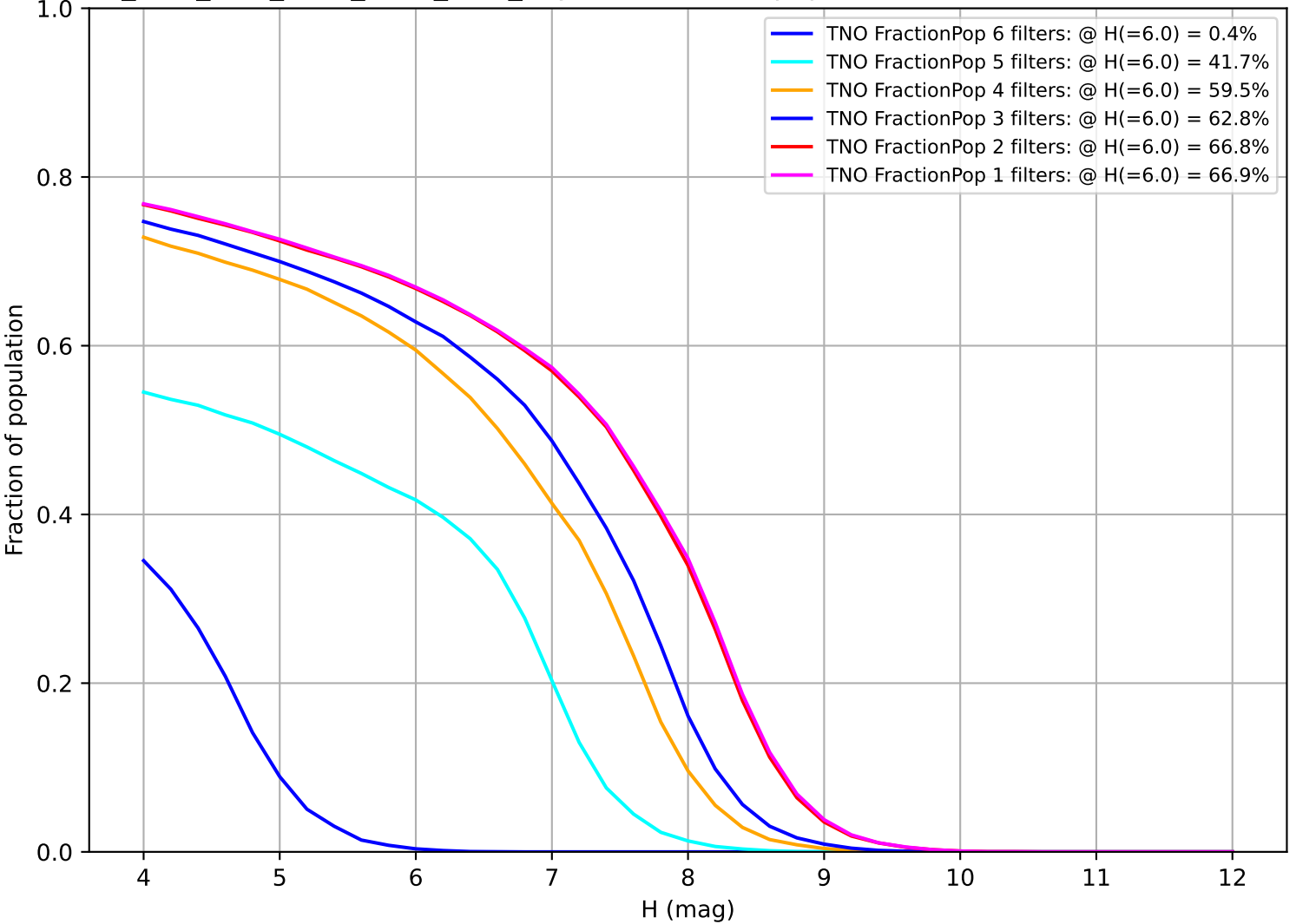
ddf_acor_sf10_lsf30_lsr20_v3.4_10yrs: Fraction of population with colors in X filters TNO
